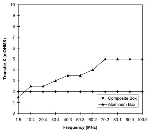
Transfer Impedance
