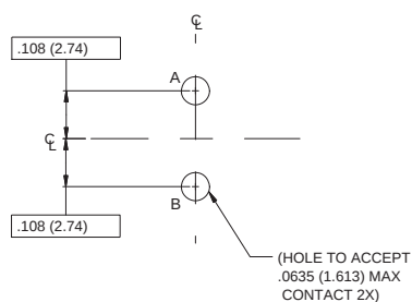
Pin Connector
