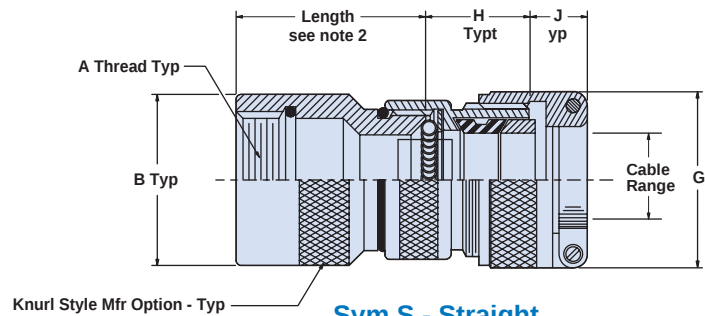
Sym S - Straight
