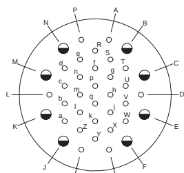
Insert Arrangement 20-38 8 #16 Contacts 30 #22 Contacts
