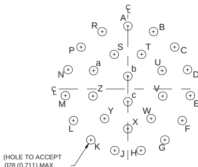
Pin Connector
