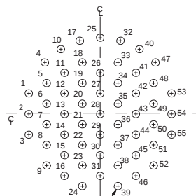
Pin Connector
