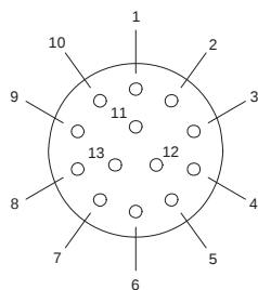
Insert Arrangement 10-13 13 #22 Contacts
