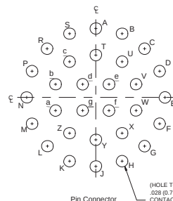
Pin Connector
