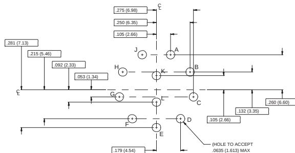
Pin Connector
