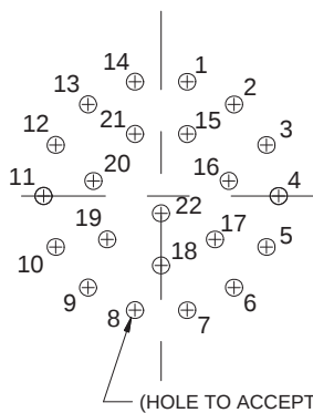
Pin Connector
