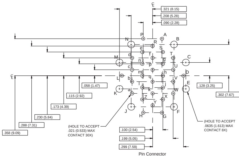
Pin Connector
