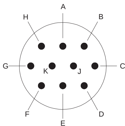
Insert Arrangement 12-10 10 #20 Contacts
