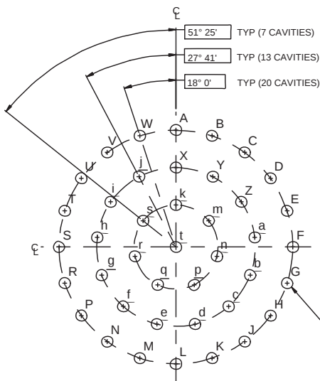
Pin Connector
