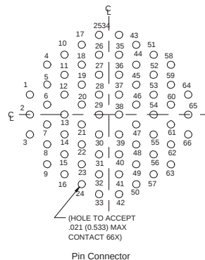
Pin Connector
