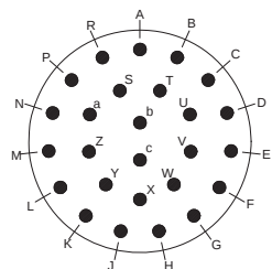
Insert Arrangement 16-26 26 #20 Contacts
