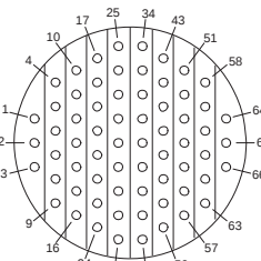
Insert Arrangement 18-66 66 #22 Contacts
