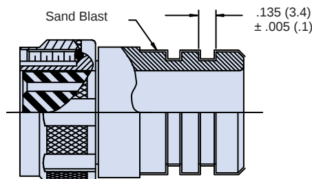
Molding Adapter Option
