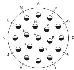
Insert Arrangement 16-19 19 #16 Contacts
