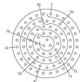
Insert Arrangement 20-79 79 #22 Contacts
