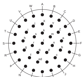
Insert Arrangement 20-41 41 #20 Contacts
