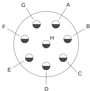
Insert Arrangement 12-08 8 #16 Contacts
