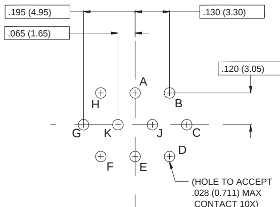
Pin Connector
