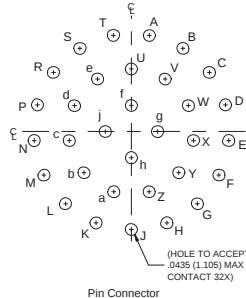
Pin Connector
