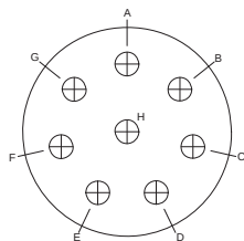
Insert Arrangement 18-8 8 #12 Contacts
