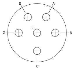
Insert Arrangement 16-6 6 #12 Contacts
