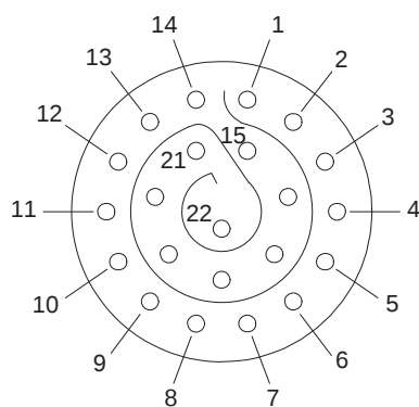
Insert Arrangement 12-22 22 #22 Contacts
