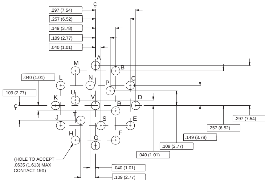
Pin Connector
