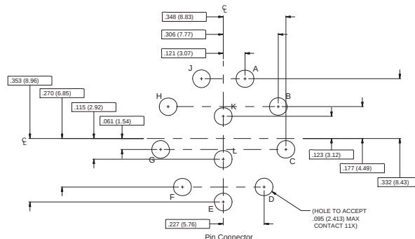
Pin Connector
