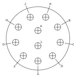
Insert Arrangement 20-11 11 #12 Contacts
