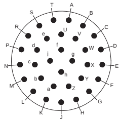
Insert Arrangement 18-32 32 #20 Contacts
