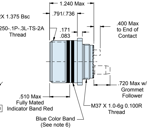
00-Wall Mount Receptacle With Slotted Holes
