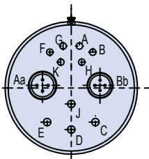
ARRANGEMENT 19Q-12 6X SIZE 20 4X SIZE 16 2X SIZE 8 QUADRIX
