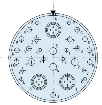
Arrangement 25Q-20 (IAW prEN 3645-001) 10 #20 Contacts 13 #16 Contacts 4 #12 Contacts 3 #8 Quadrax Contacts (J1)
