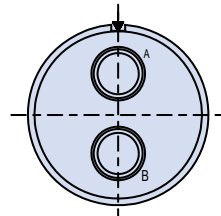
ARRANGEMENT 17Q-75 (IAW PREN 3645-001) 2X SIZE 8 QUADRIX
