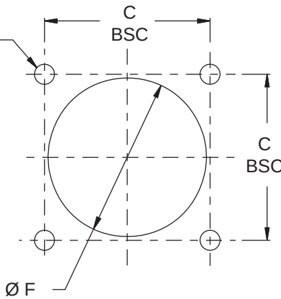
Square Flange Front Panel Mount
