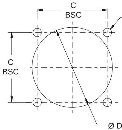
Square Flange Back Panel Mount
