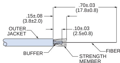
Pin Terminus 181-057
