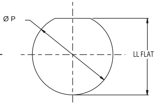
Recommended Panel Cut-Out Jam-Nut Mount
