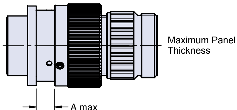
Panel thickness for type 03 FF and 030 connectors
