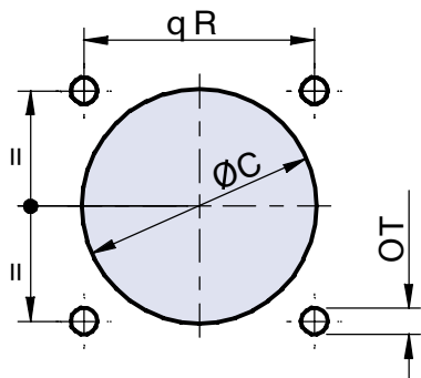
Panel cutout for type 03 FP connectors (front panel mounting)
